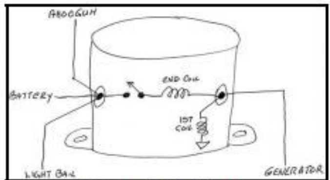
Cut-out electrical circuit
